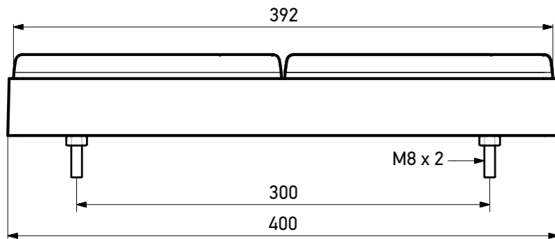
General Dimensions (in millimetres)
