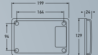
Jumbo-S LED Reversing Lamp 2ZR 980 762-031 (1461)
